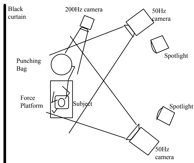
Figure 5. Overhead diagram of the data collection set-up.
