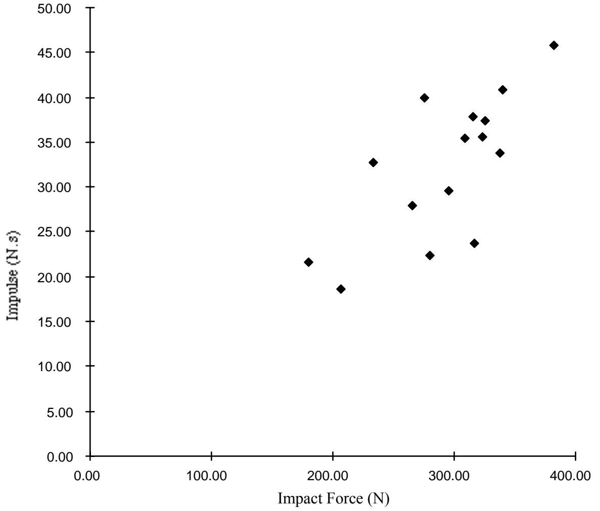
Figure F1. Plot of impulse against impact force
